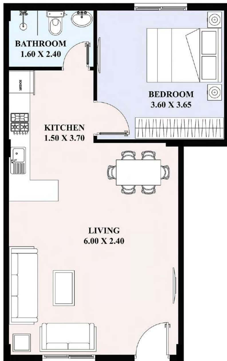
1B/Simplex / TYPE B GROUND FLOOR
